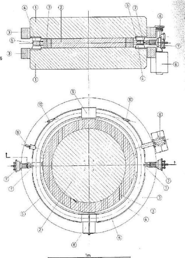
Fig. 1. - Elevation and plan section of the Frascati Storage Ring (anello di accumulazione - AdA): 1) magnet pole; 2) magnet core; 3) coils; 4) polepieces; 5) doughnut; 6) transverse pump; 7) injection ports; 8) RF cavity; 9) experimental section; 10) windows for the observation of the synchrotron radiation; 11) vacuum gauge.
