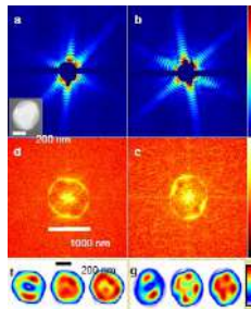
Imaging single mimivirus Seibert et al, Nature, 470, 78 (2011)
