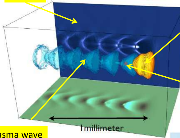
Plasma Cavity
